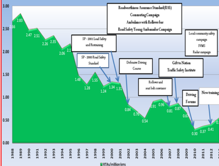
MVI's/million kms
