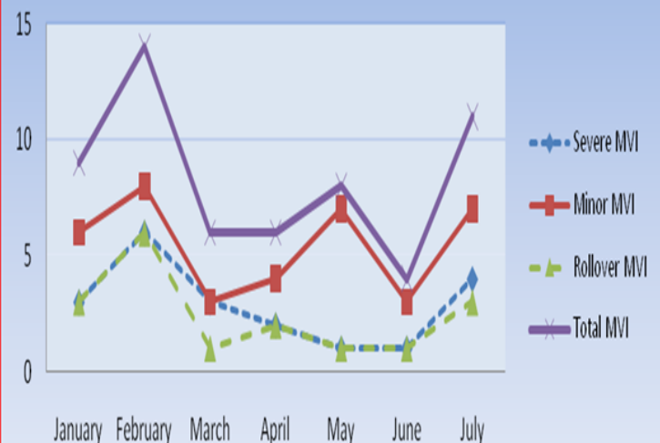
MVI Statistics 2014
